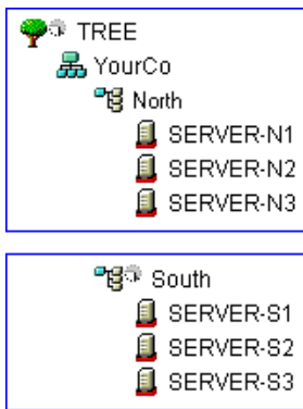
Figure 1-17 Sample Partitions
