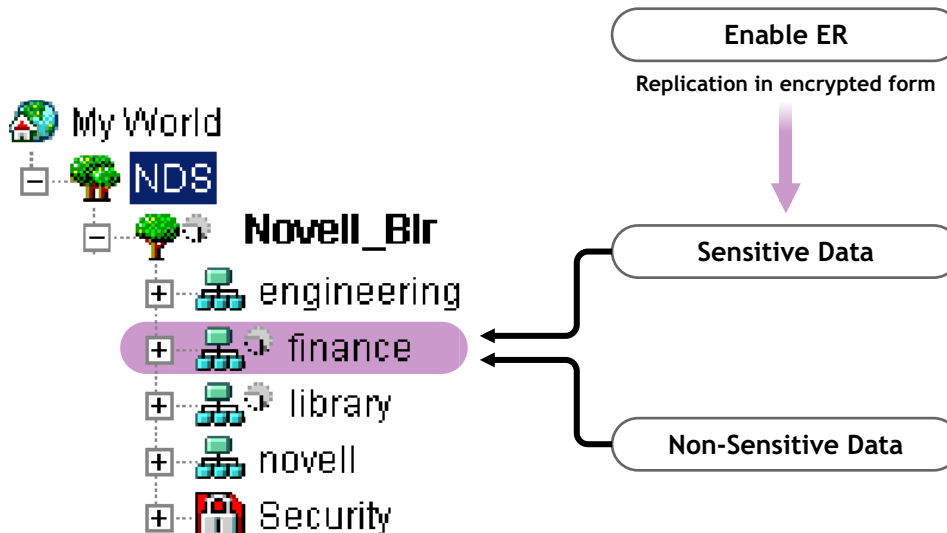
Figure 11-3 Encrypted Replication
