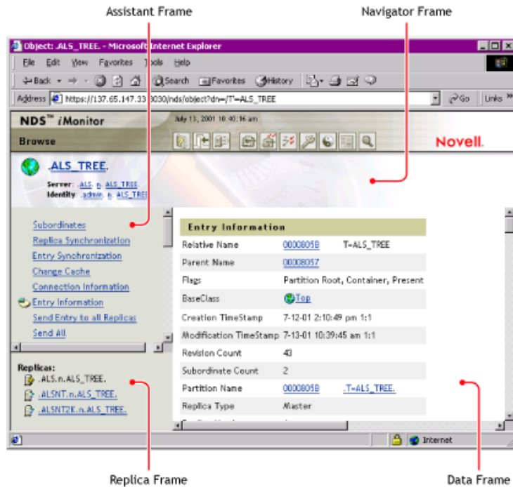
Figure 8-1 iMonitor Frames
