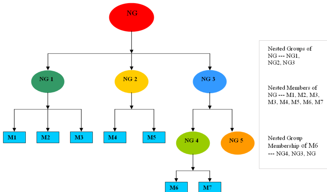
Figure 1-5 Nested Groups
