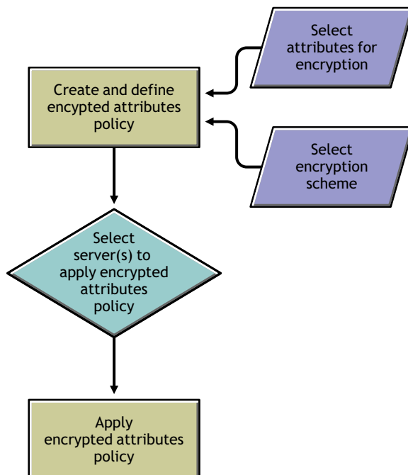
Figure 11-2 Encrypting Attributes
