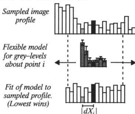
Figure 2. Suggested movement of point dX_i is along normal to boundary, in a direction towards the point at which the profile model best fits the profile sampled from the image.
